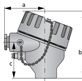
AXD (aluminium, Ex, IP68)
